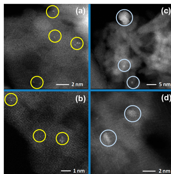
Figure 3. STEM images from a 0.1% Ru/Al 2 O 3 catalyst before (images a and b) and after (images c and d) CO 2 reduction at 350 °C for 16 h.
