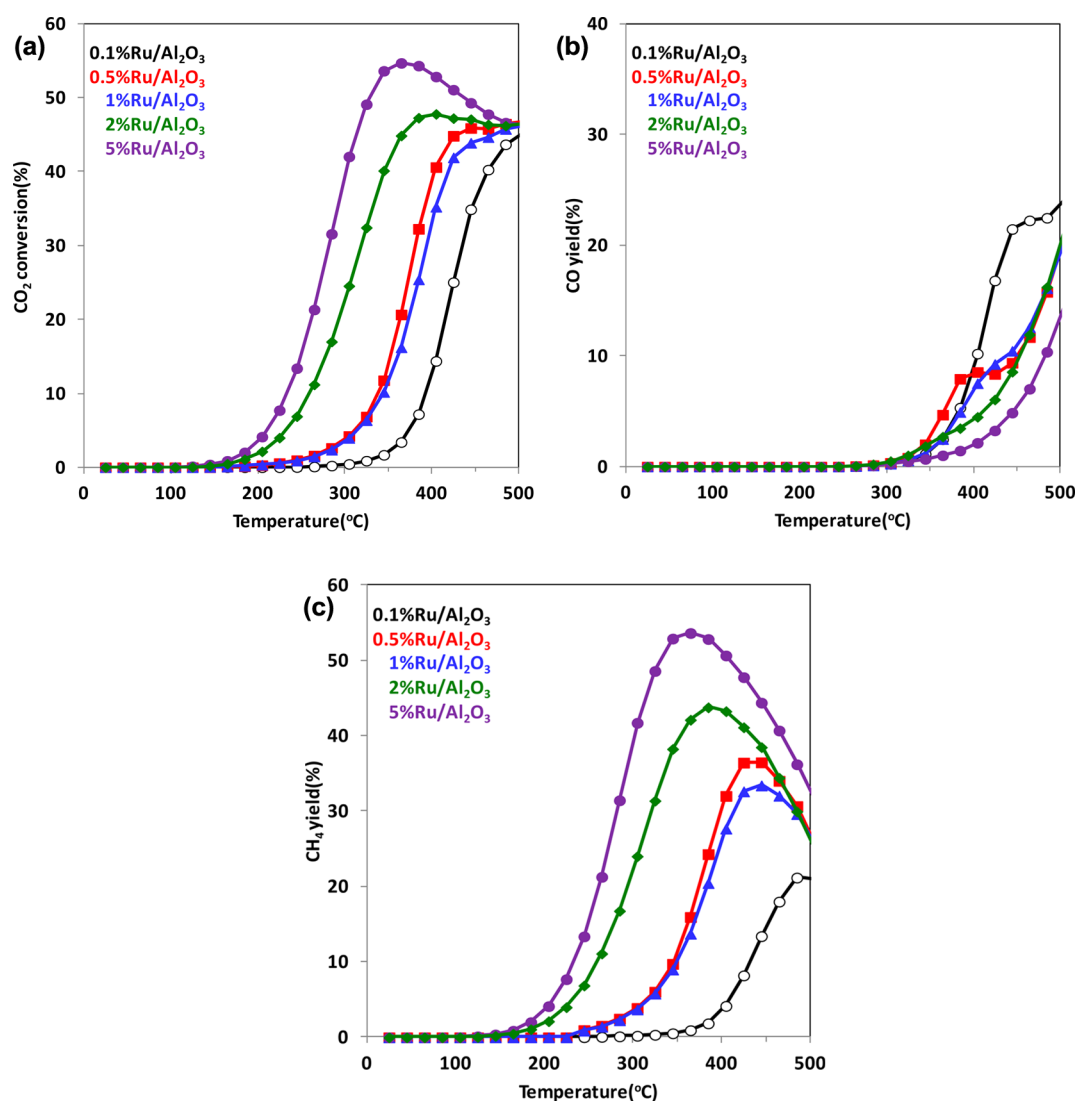
Figure 1. Temperature programmed \text{CO}_2 reduction reaction on \text{Ru}/\text{Al}_2\text{O}_3 catalysts: \text{CO}_2 conversion (a) and \text{CO} (b) and \text{CH}_4 (c) yields. ( m_{\text{catalyst}} = 50 mg, 5% \text{CO}_2 + 15\% \text{H}_2 in He (total flow rate = 60 mL/min), heating rate = 5 ^\circ\text{C}/\text{min} .)
