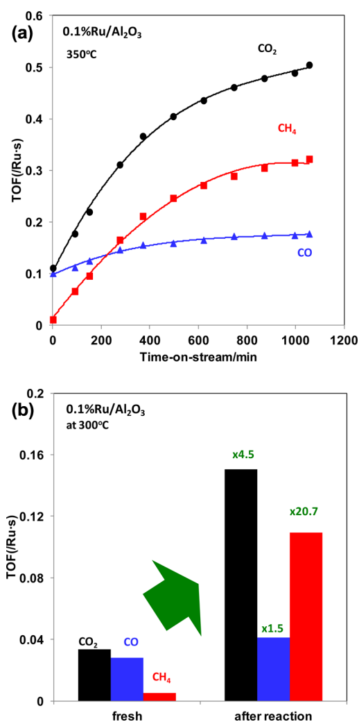
Figure 2. (a) TOFs of CO 2 , CO, and CH 4 as a function of time-on-stream at 350 °C over a 0.1% Ru/Al 2 O 3 catalyst. (b) Steady state TOFs for CO 2 conversion and CO/CH 4 production over a fresh and reactivated (after reaction at 350 °C) 0.1% Ru/Al 2 O 3 catalyst at 300 °C.
